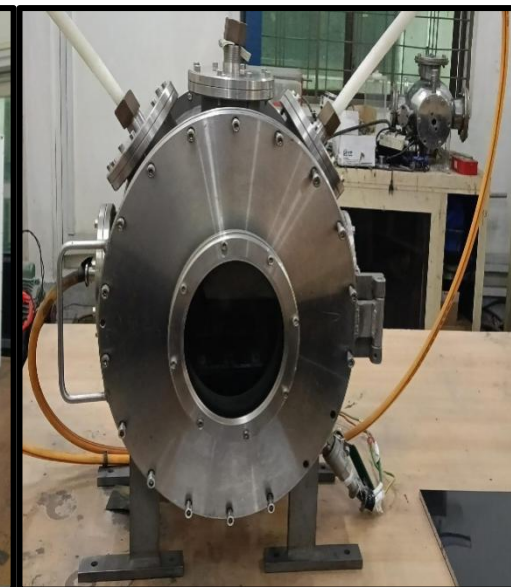
Plasma Chamber
