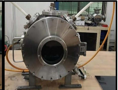
Plasma Chamber
