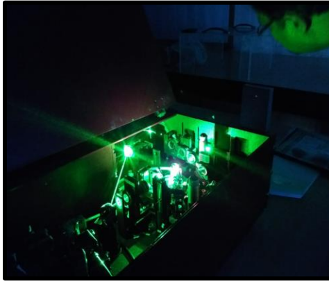
Femtosecond
