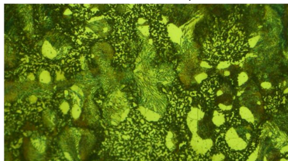
Microstructure of Gray Cast Iron
